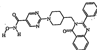
compound 10 .CF 3 COOH
